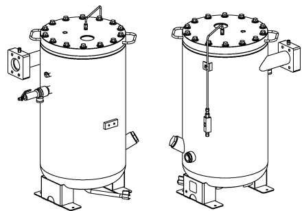
ASSEMBLED VIEWS
